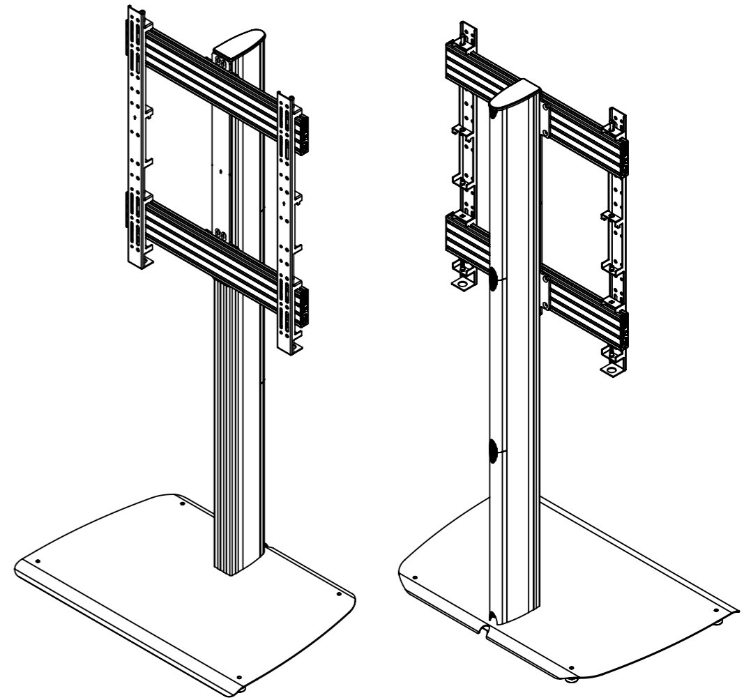
ISOMETRIC VIEW
